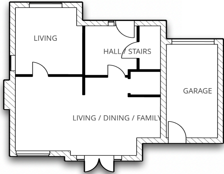
Ground Floor Scale - 1:50
