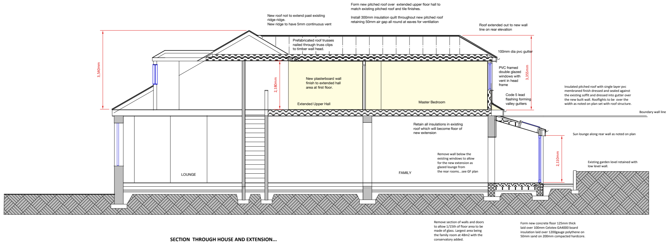
SECTION THROUGH HOUSE AND EXTENSION...
