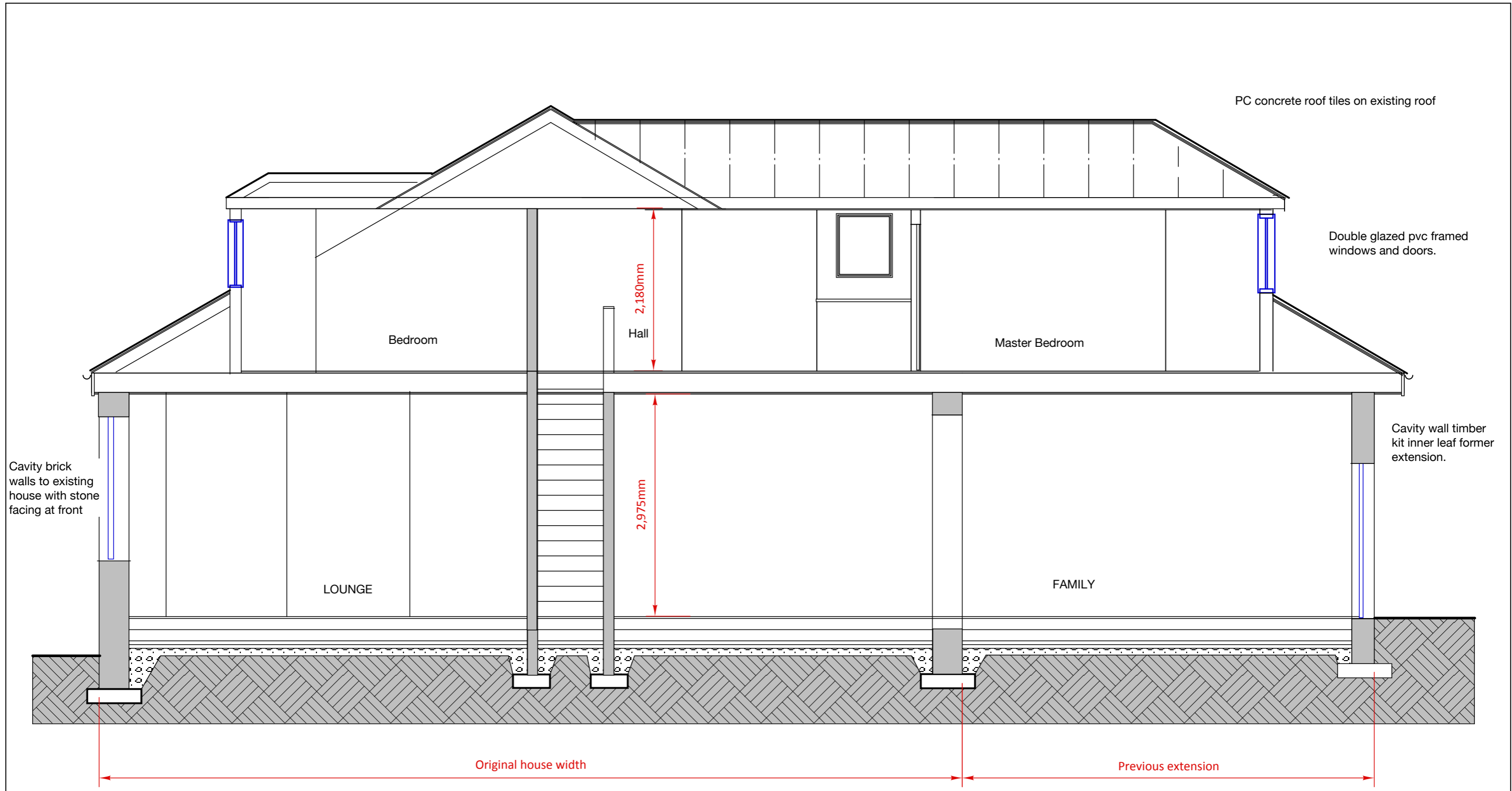
SECTION THROUGH EXISTING HOUSE...
