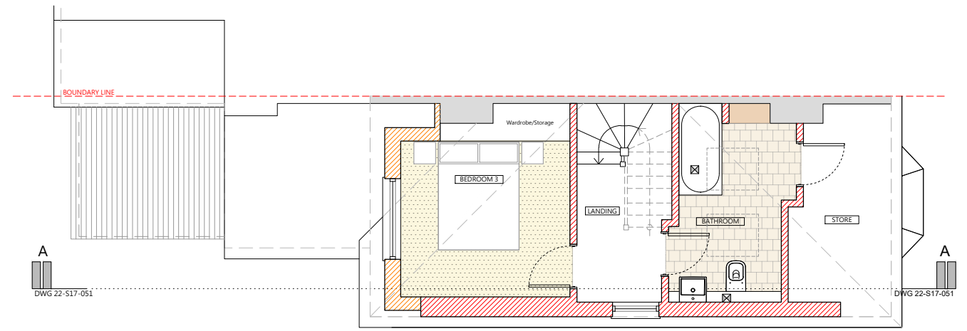
Second Floor Plan Scale 1:100 @ A3
