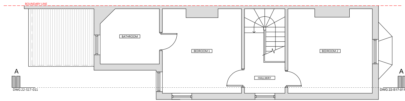
First Floor Plan Scale 1:100 @ A3
