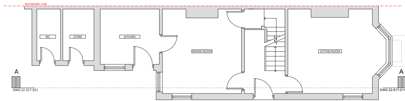
Ground Floor Plan Scale 1:100 @ A3
