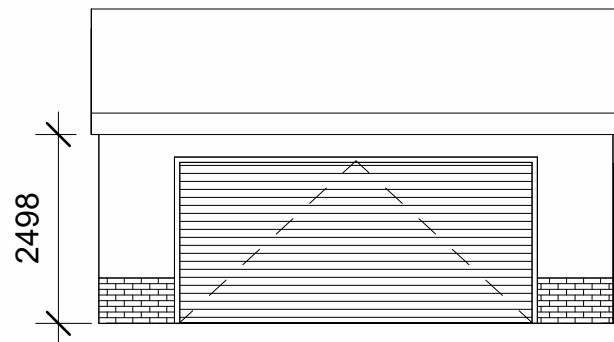
3 Proposed Front Elevation 1 : 100
