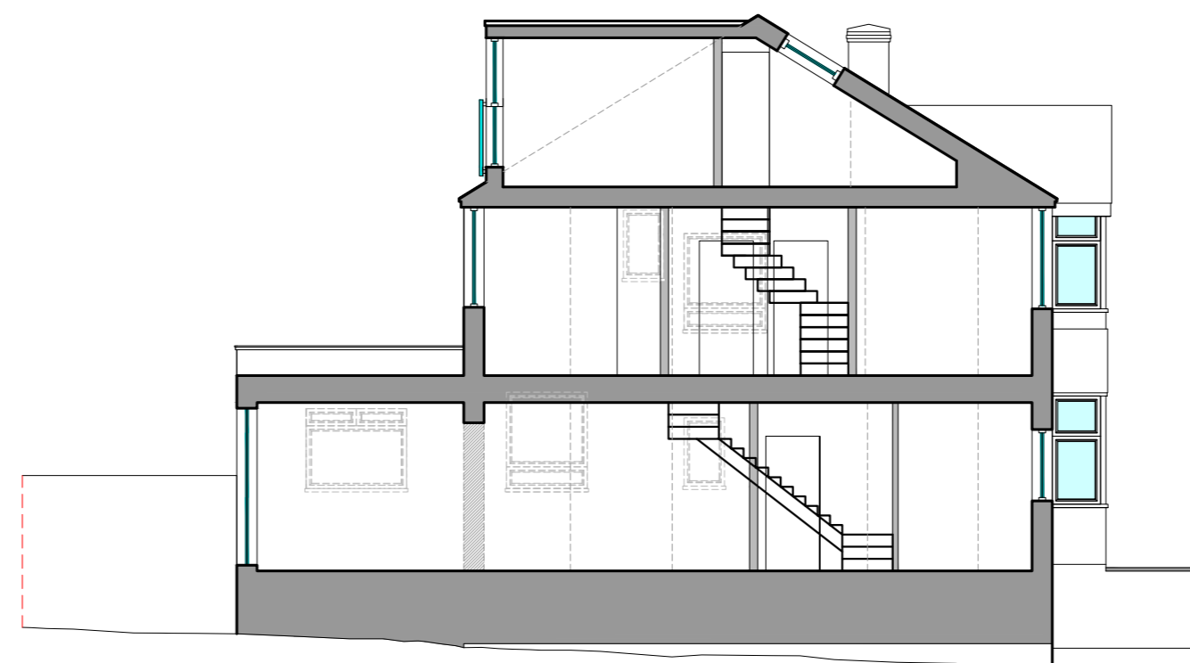
SECTION, PROPOSED PLAN, SCALE 1:100
