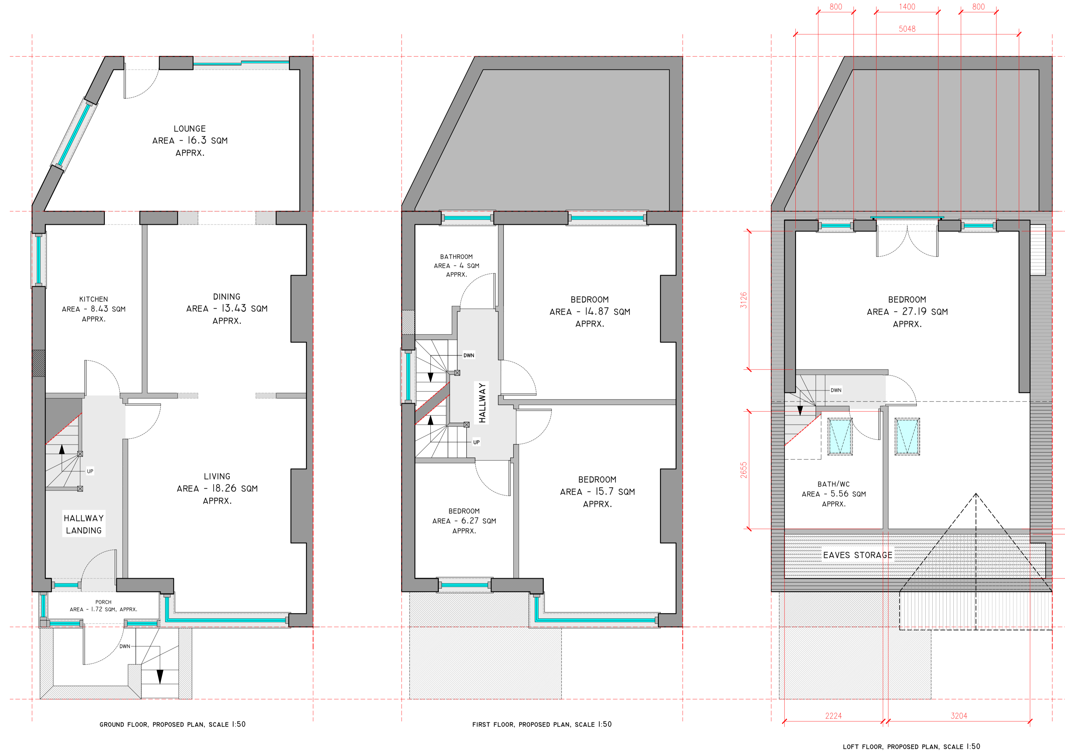
LOFT FLOOR, PROPOSED PLAN, SCALE 1:50
