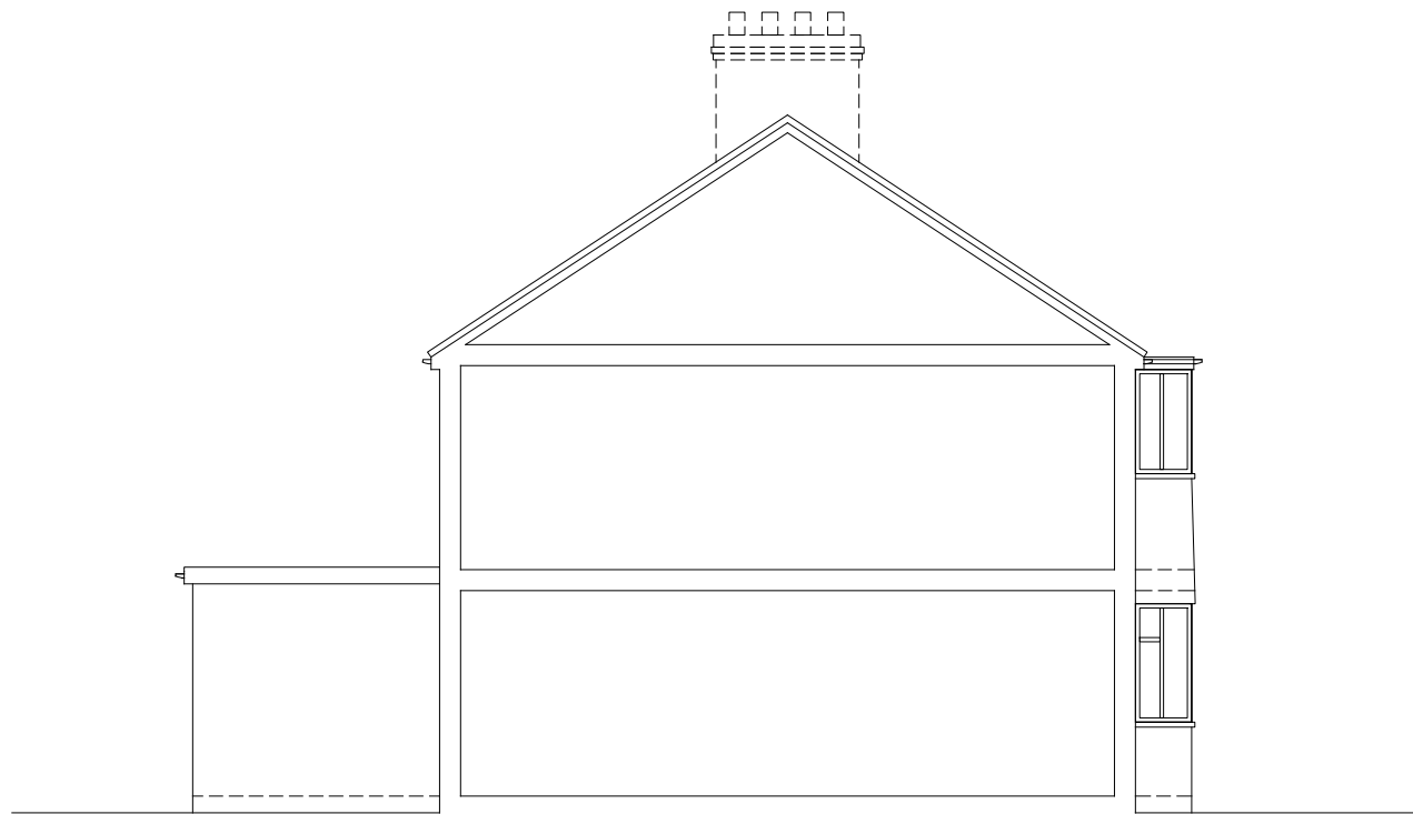
EXISTING LEFT SIDE ELEVATION 1:100
