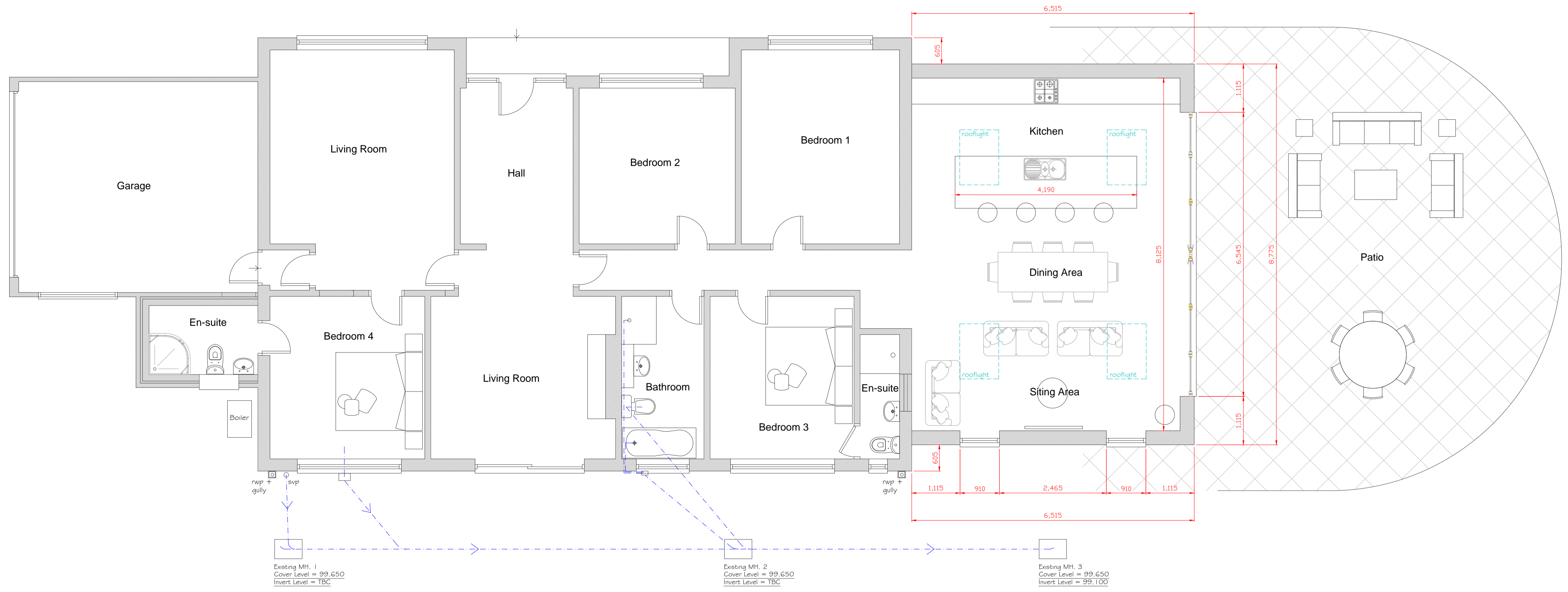
Proposed Floor Plan 1:50
