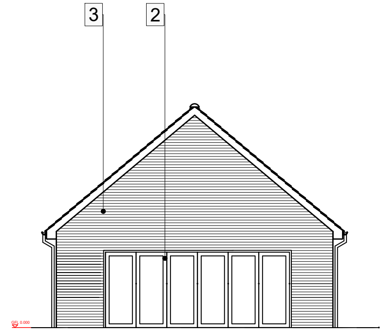
REAR ELEVATION
