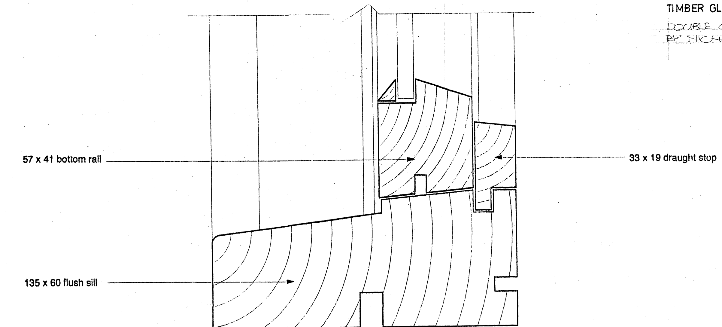
Typical Vertical Section. 1 : 1. Patent Stormproofing seals to meeting rails and sash framing by window manufacturer
