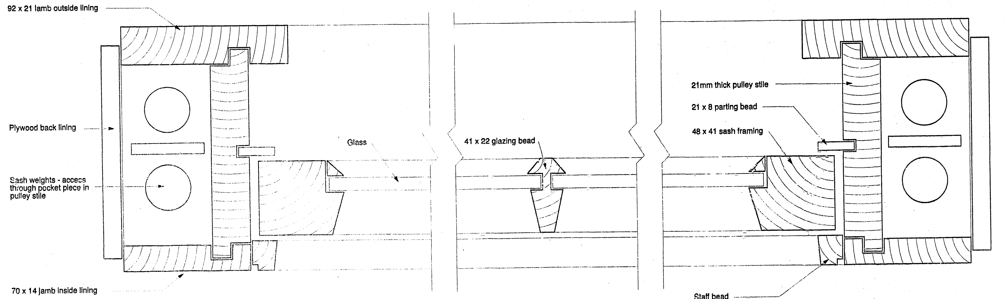
Typical Horizontal Section 1 : 1. Patent Stormproofing seals to meeting rails and sash framing by window manufacturer
