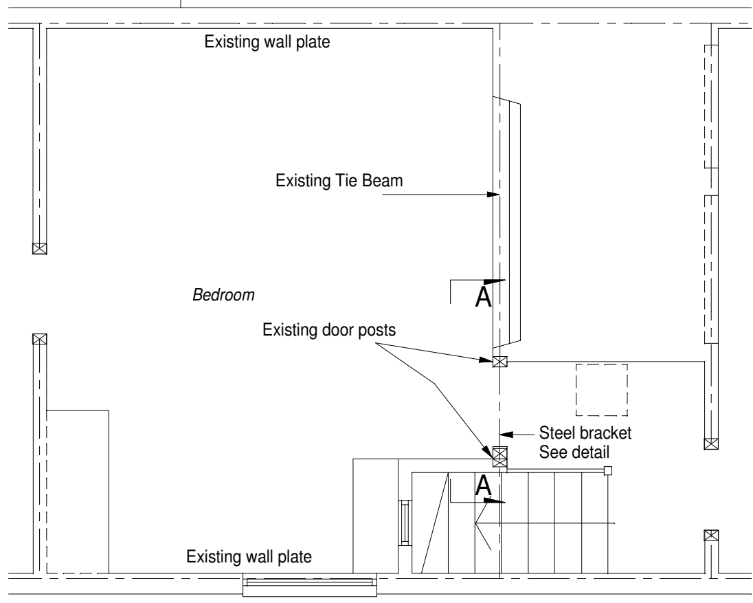
Part-First Floor Plan @ 1:50
