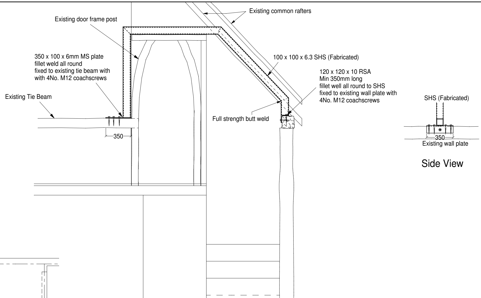
Section A-A @ 1:25
