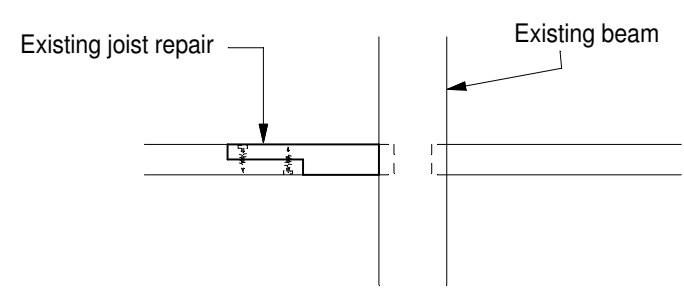
Typical Joist Repair Detail -Plan View Over Sitting Room
