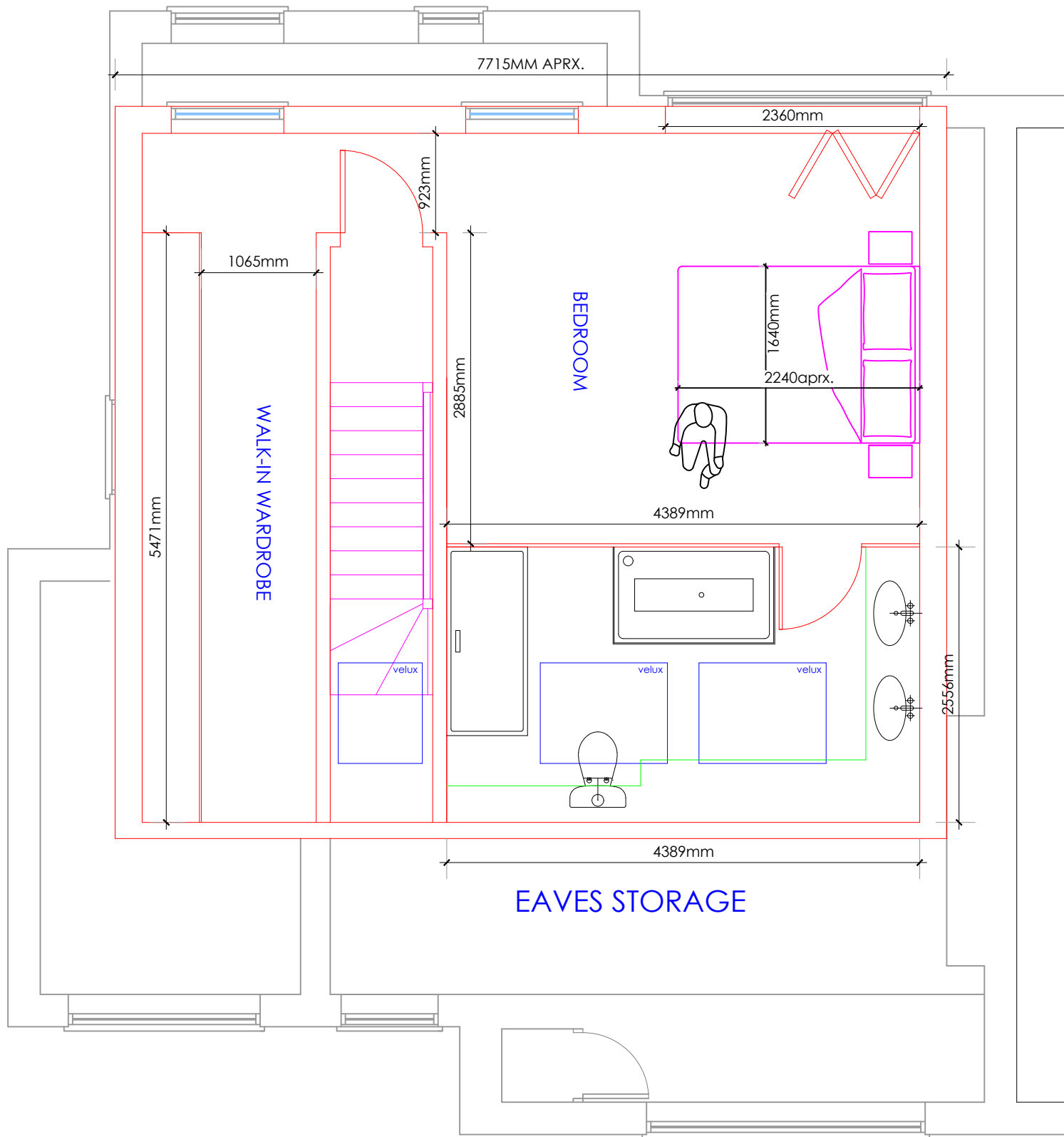
PROPOSED SECOND FLOOR PLAN Scale 1:50 @ A3 N 0 500 1000 1500 2000 SCALE (MM)
