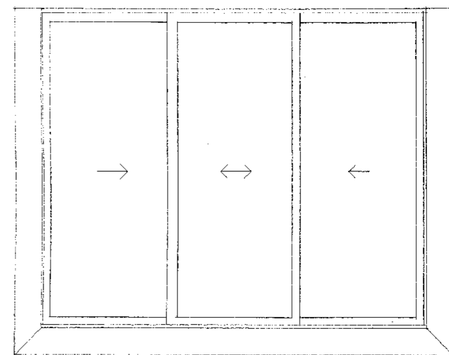
INTERNAL GLAZING ELEVATION 1:20
