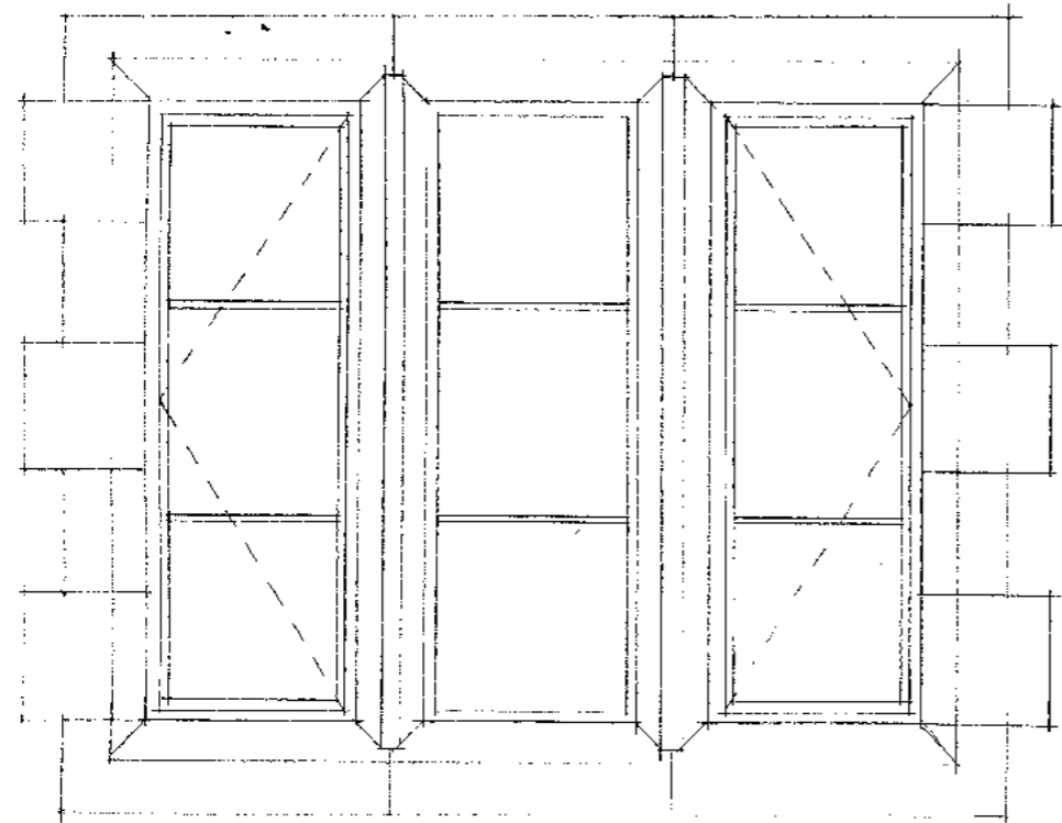
EXTERNAL ELEVATION 1:20 (no change)
