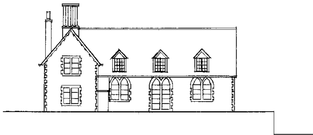
WEST ELEVATION 1:200
