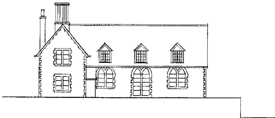
WEST ELEVATION 1:200
