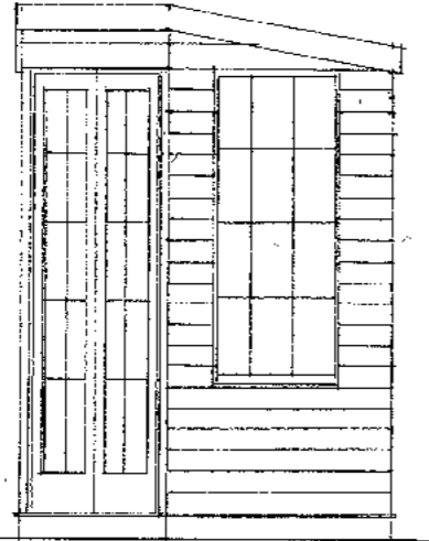
SOUTH ELEVATION 1:20
