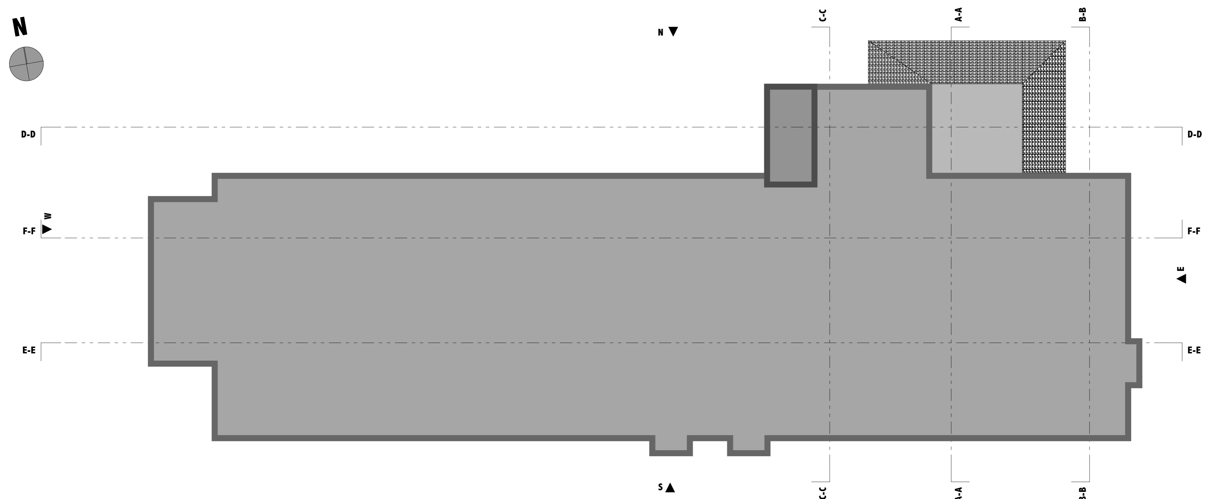
EXISTING ROOF PLAN SCALE 1:100
