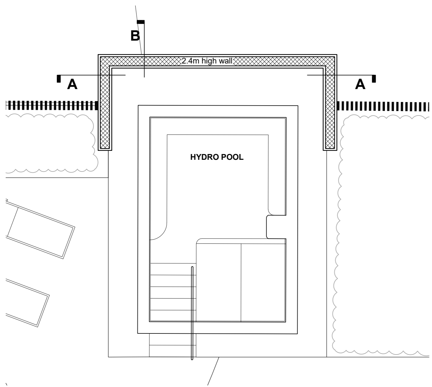
SPA GARDEN WALL HYDRO POOL - PLAN
