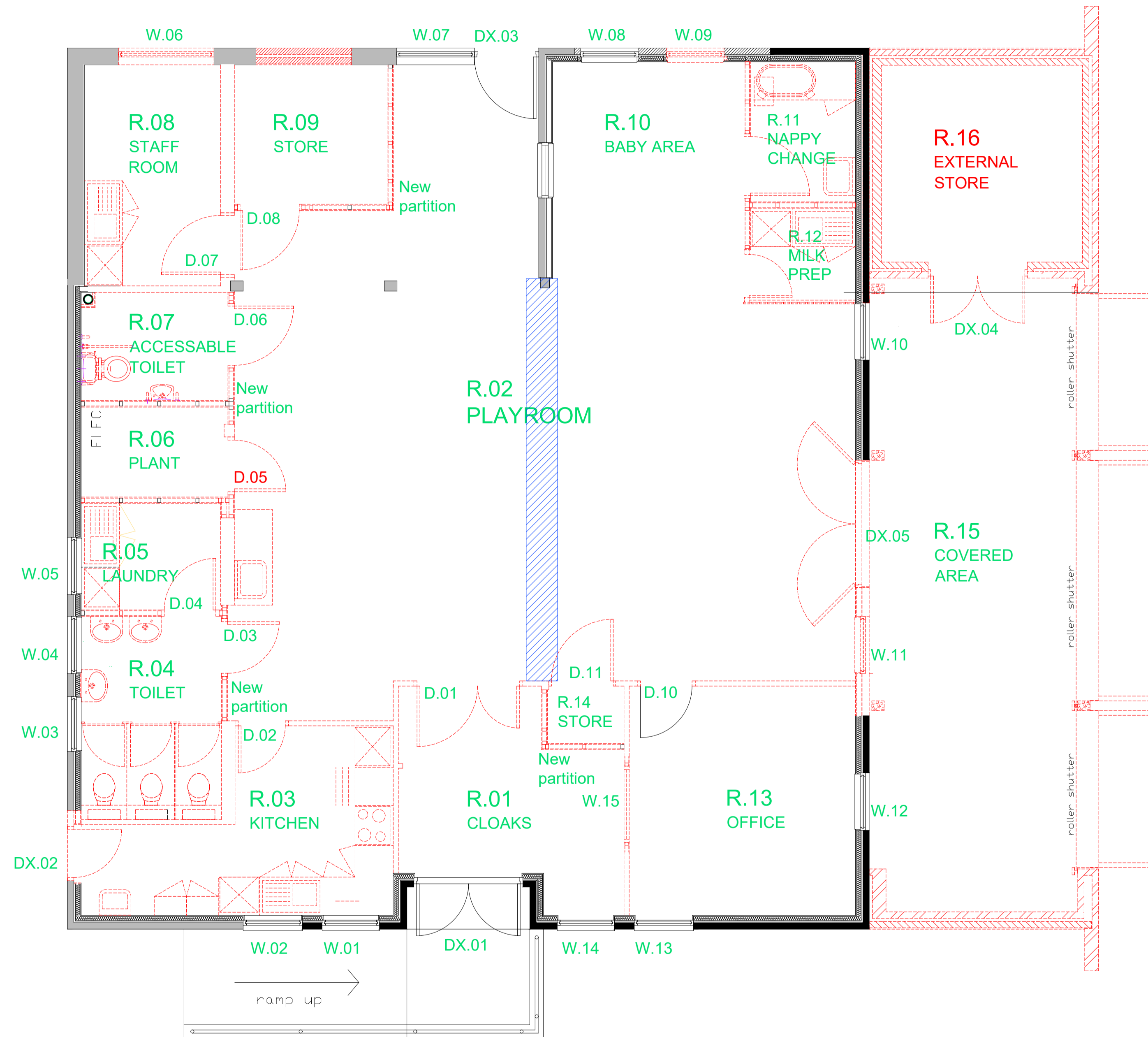
DEMOLITION GROUND FLOOR PLAN
