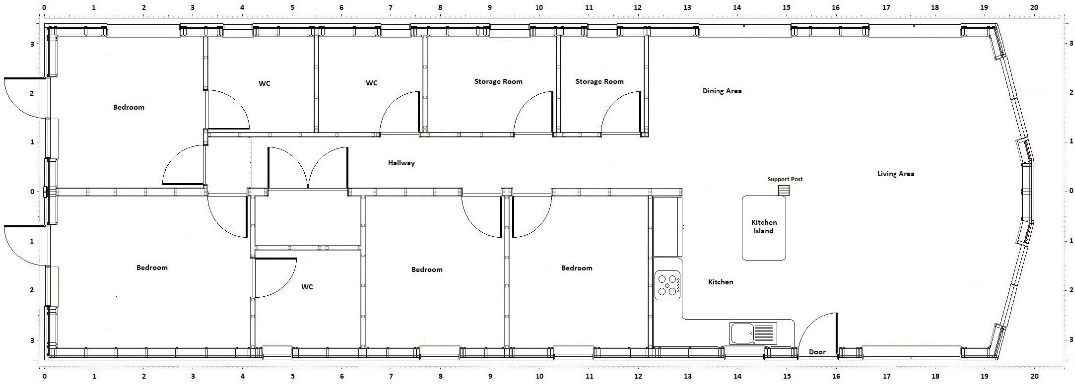
INDICATIVE ACCOMMODATION UNIT LAYOUT
