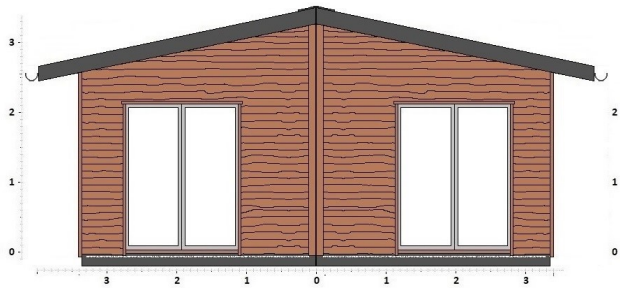
Indicative Rear Elevation
