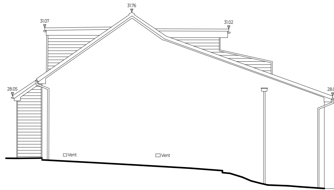
WEST ELEVATION 1:100
