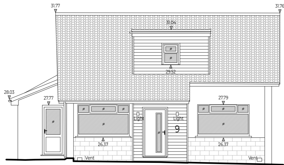
NORTH ELEVATION 1:100
