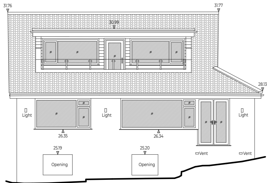
SOUTH ELEVATION 1:100
