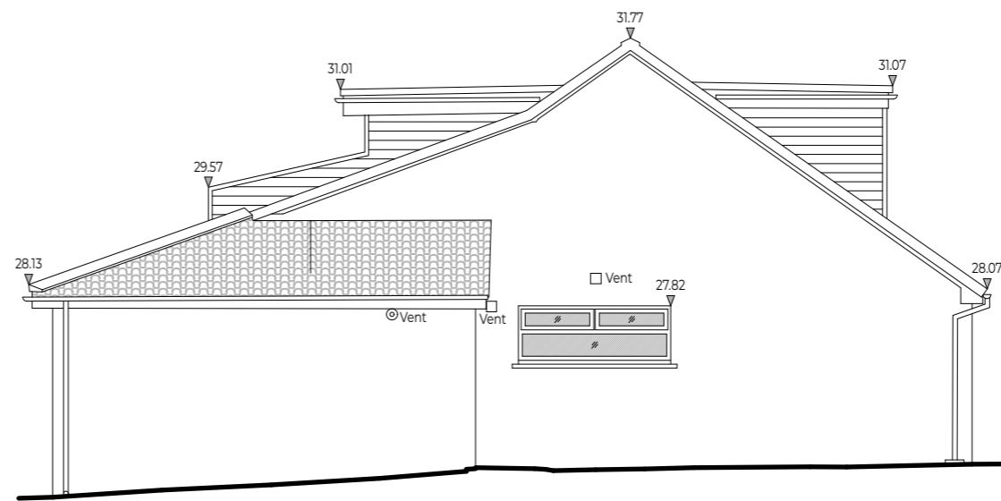
EAST ELEVATION 1:100
