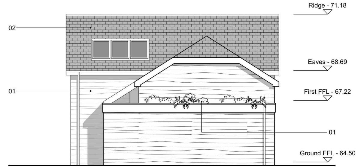
02 Proposed East Elevation 1:100
