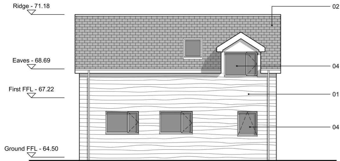
03 Proposed West Elevation 1:100
