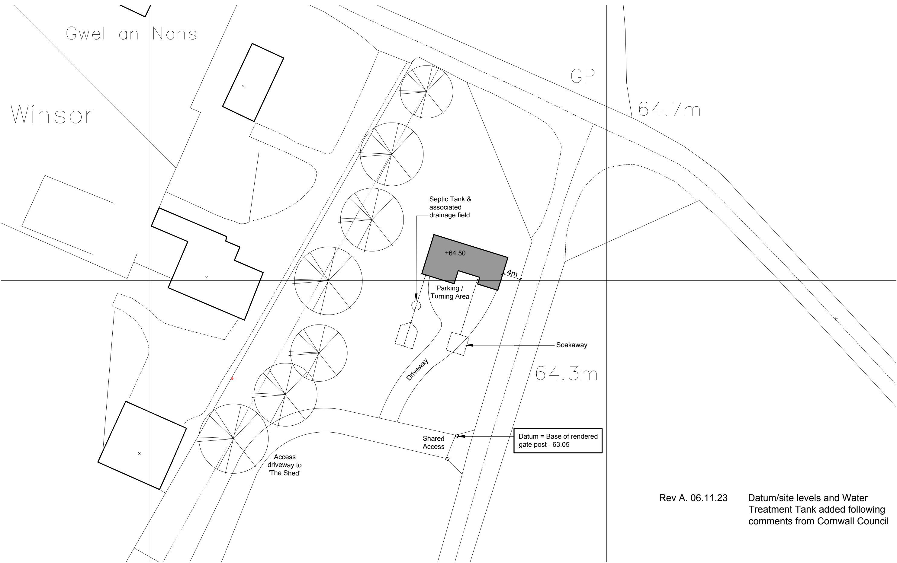
01 Proposed Block Plan 1:500
