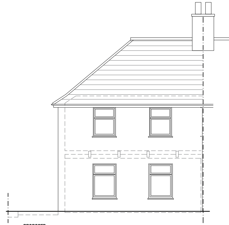
PROPOSED SOUTH ELEVATION - FRONT
