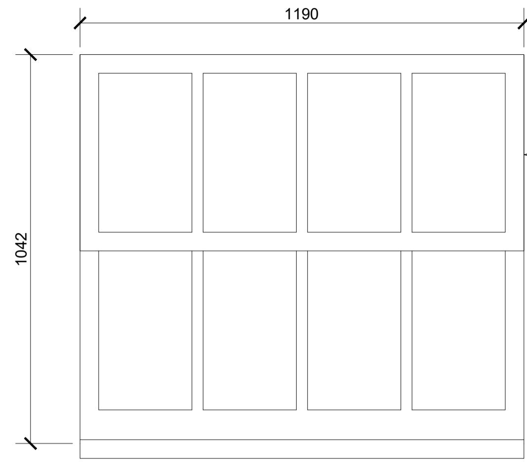
W13 GROUND FLOOR SIDE/REAR SLIMLINE DOUBLE GLAZING AT THE REAR & SINGLE GLAZING AT THE SIDE
