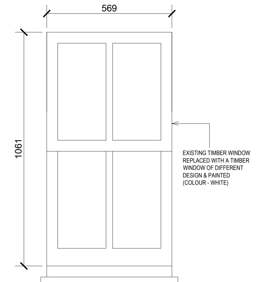
W17 BASEMENT FLOOR SIDE SINGLE GLAZING
