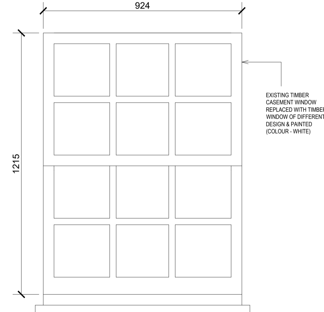
W23 GROUND FLOOR FRONT SINGLE GLAZING
