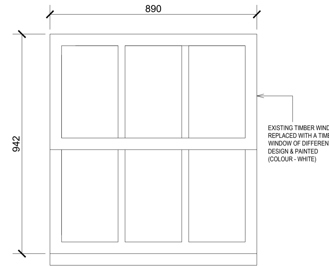
W16 GROUND FLOOR SIDE SINGLE GLAZING
