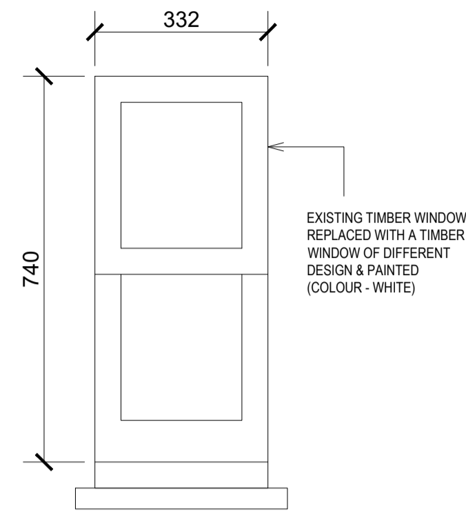
W14 SECOND FLOOR SIDE SINGLE GLAZING
