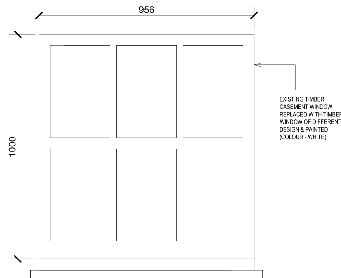
W19 ROOF SIDE SINGLE GLAZING
