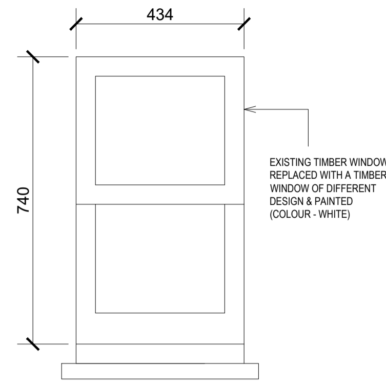
W15 GROUND FLOOR SIDE SINGLE GLAZING
