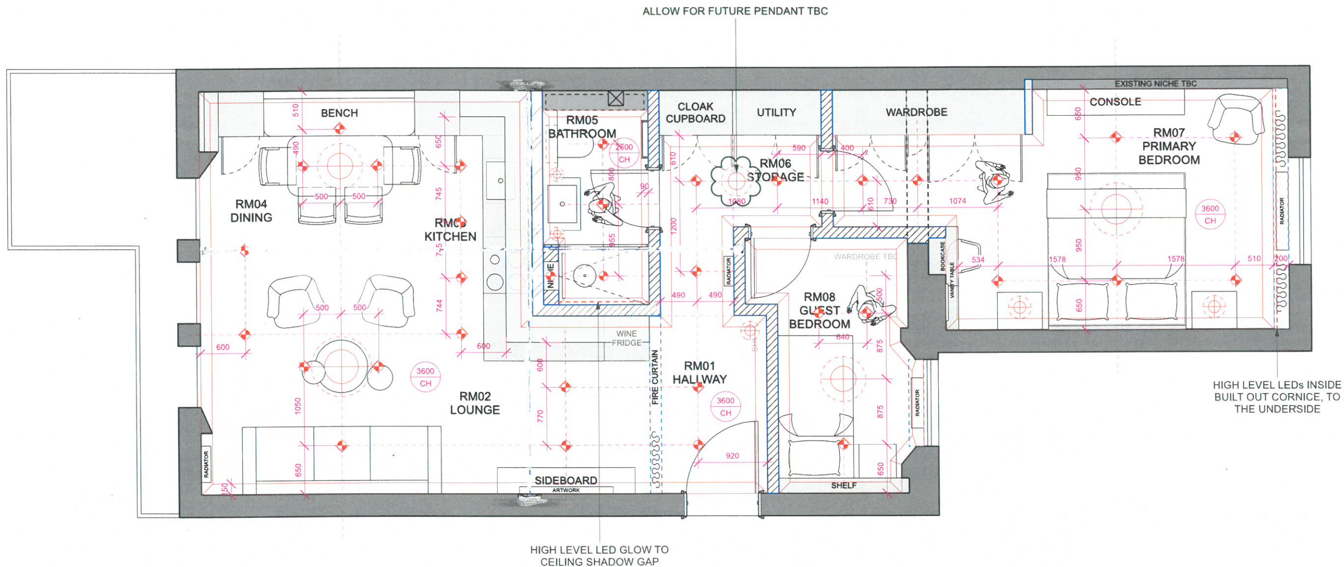
01 REFLECTED CEILING PLAN Scale: 1:50
