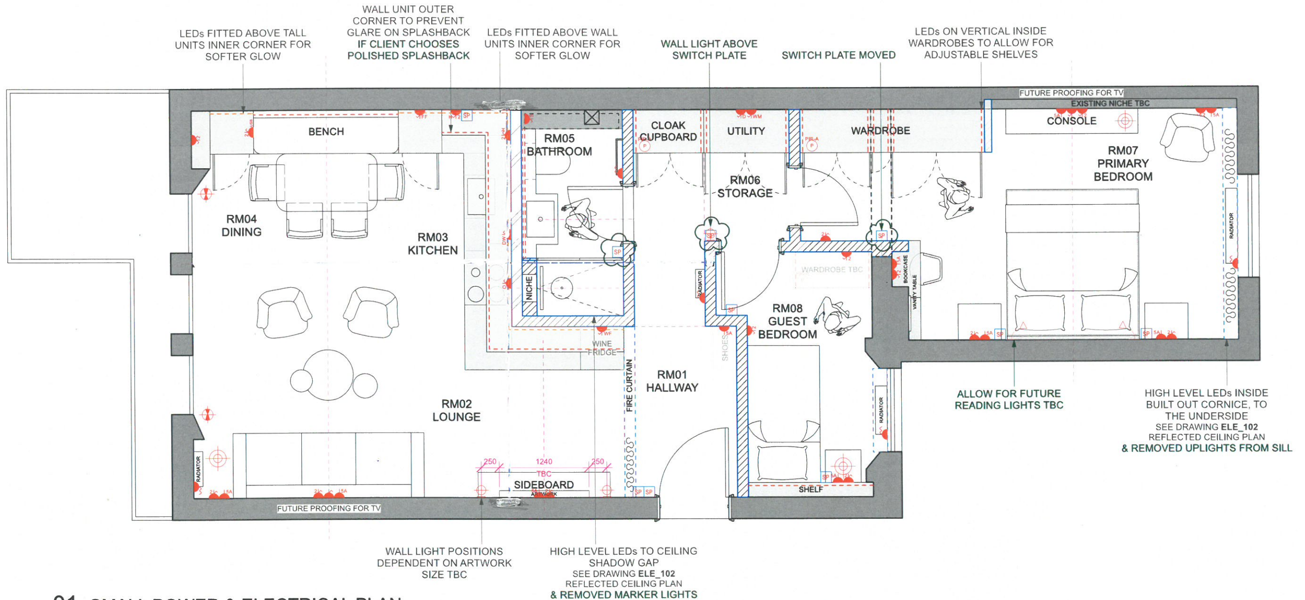
01 SMALL POWER & ELECTRICAL PLAN Scale: 1:50
