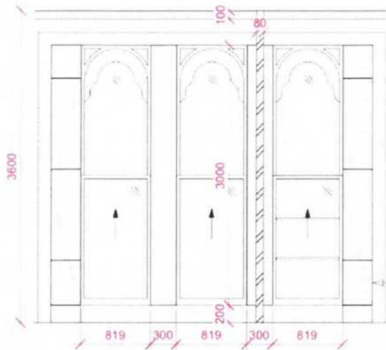
W01 KITCHEN WINDOWS Scale: 1:40
