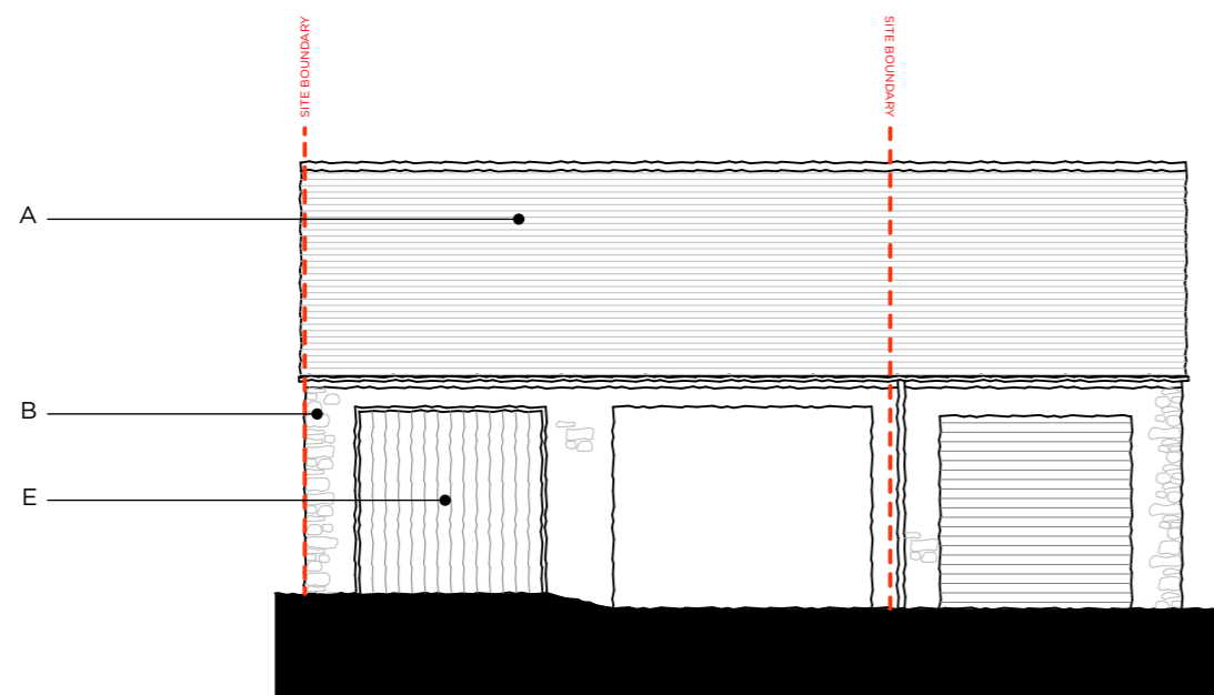
E5 Existing West Carport Elevation 1:100
