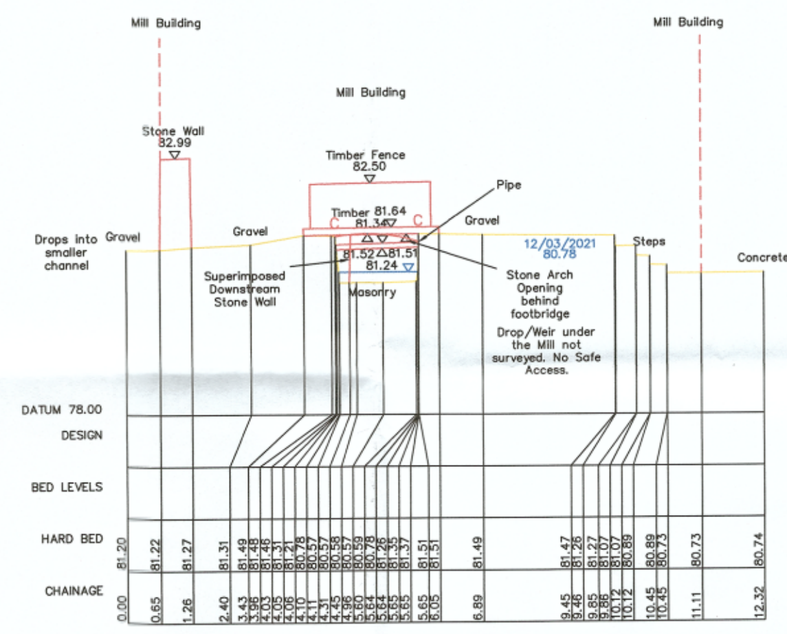
XS2 427555.25mE 204884.81mN Brg 197 Chainage 26.8 Upstream Face of Timber Footbridge. Footbridge Length 1m.
