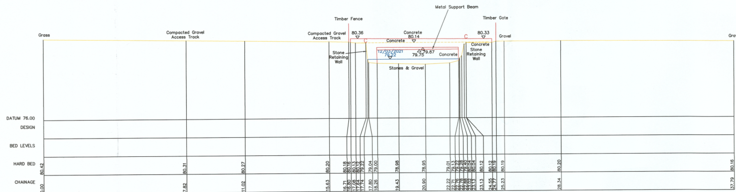
XS1 427577.18mE 204898.61mN Brg 172 Chainage 0 Upstream Face of Concrete Access Bridge. Bridge Length 4m.
