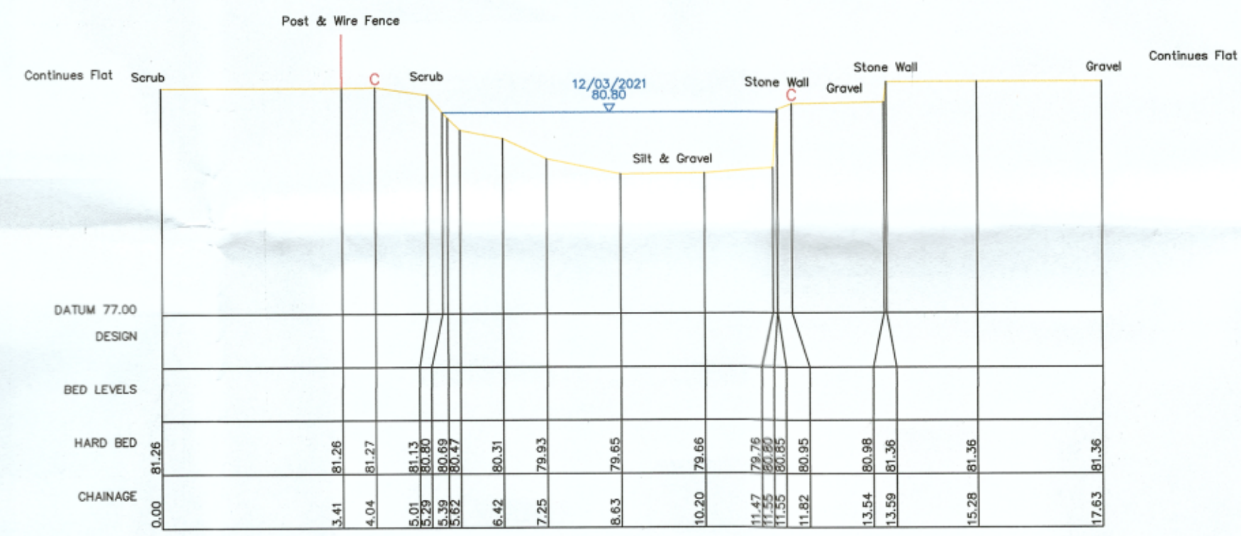
XS3 427545.39mE 204891.46mN Brg 208 Chainage 39.8 Open Channel
