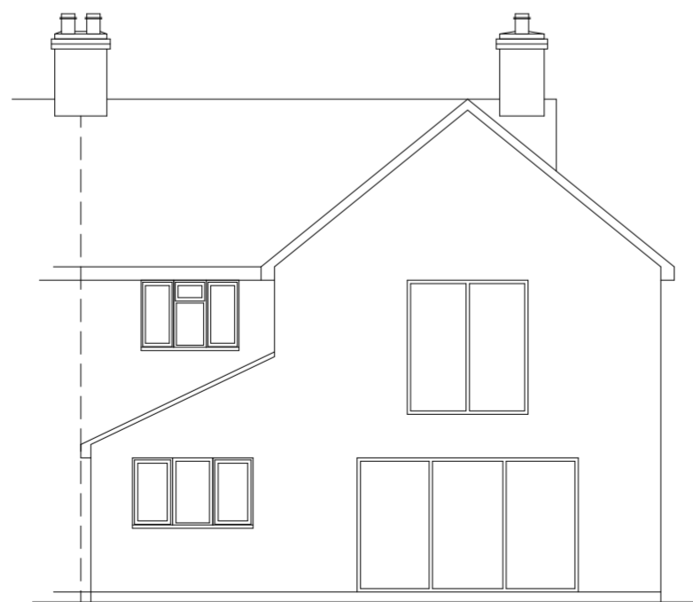
Proposed Rear
