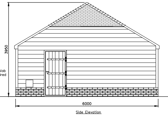
Existing Side Elevation (North)
