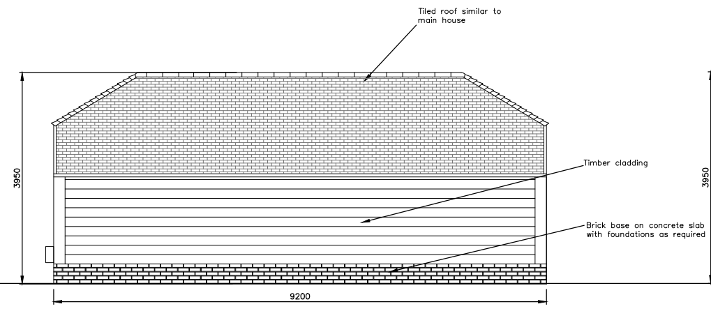
Existing Rear Elevation (West)
