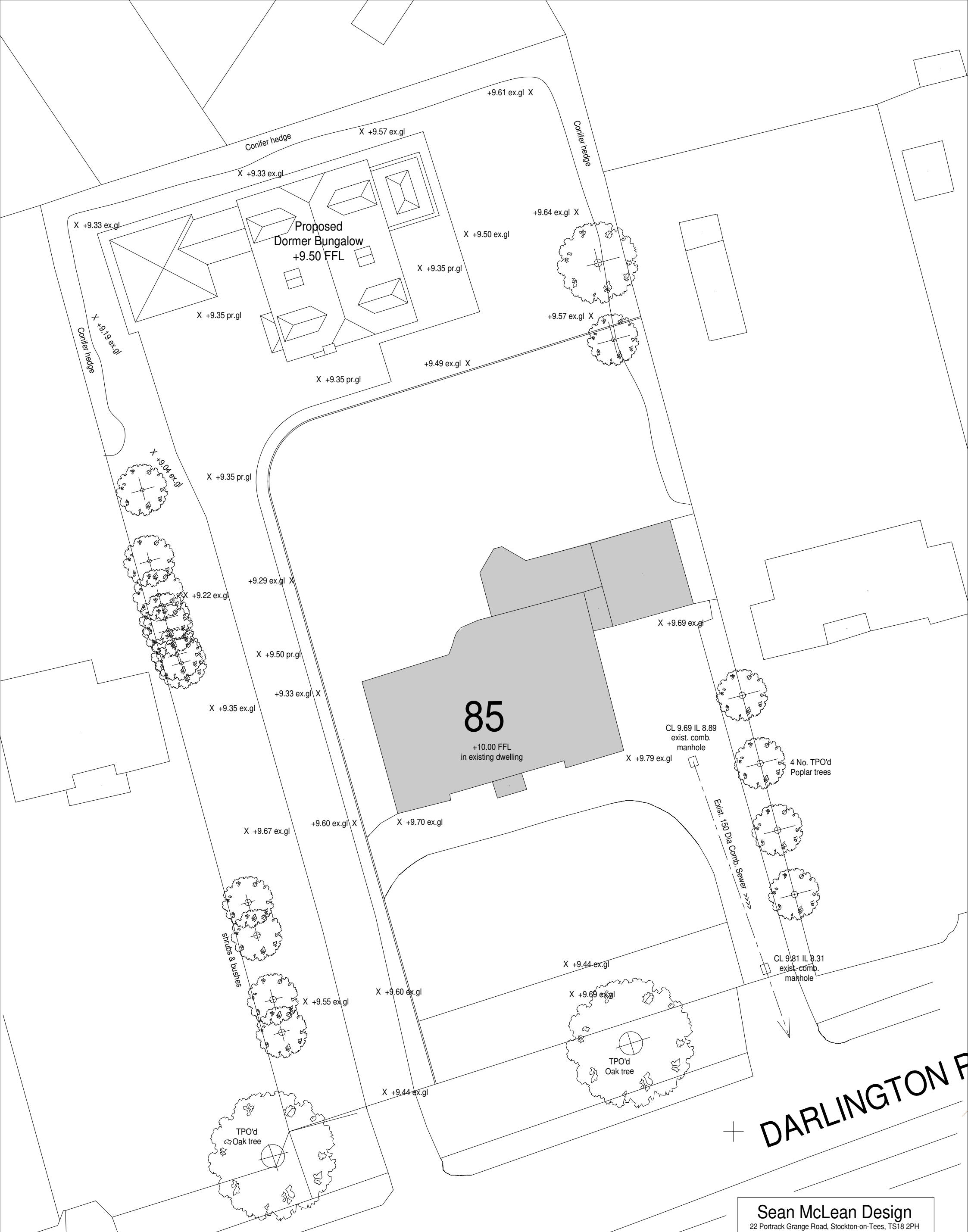
Proposed Site Levels Plan ( scale 1:250@A3 )
