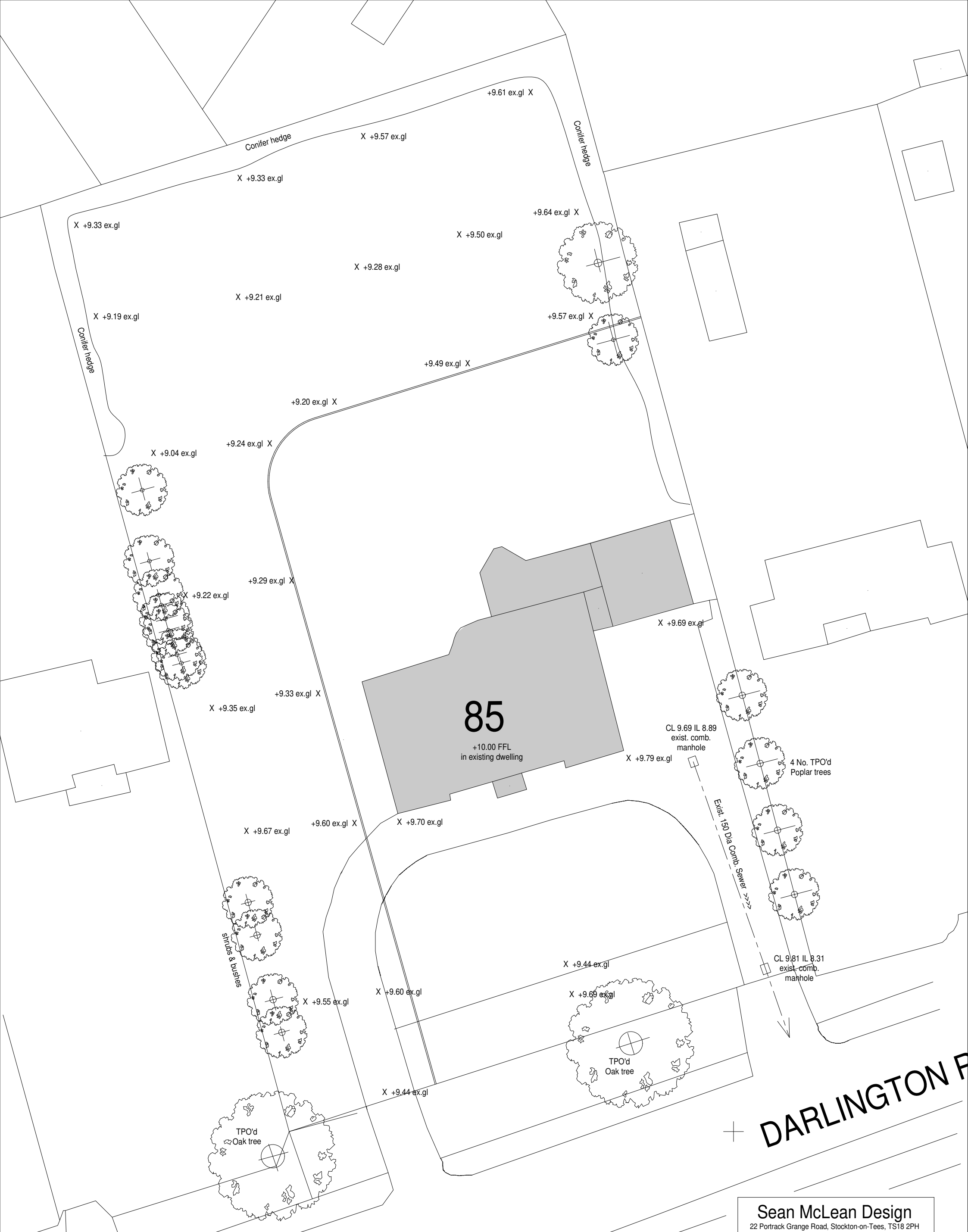
Existing Site Levels Plan ( scale 1:250@A3 )
