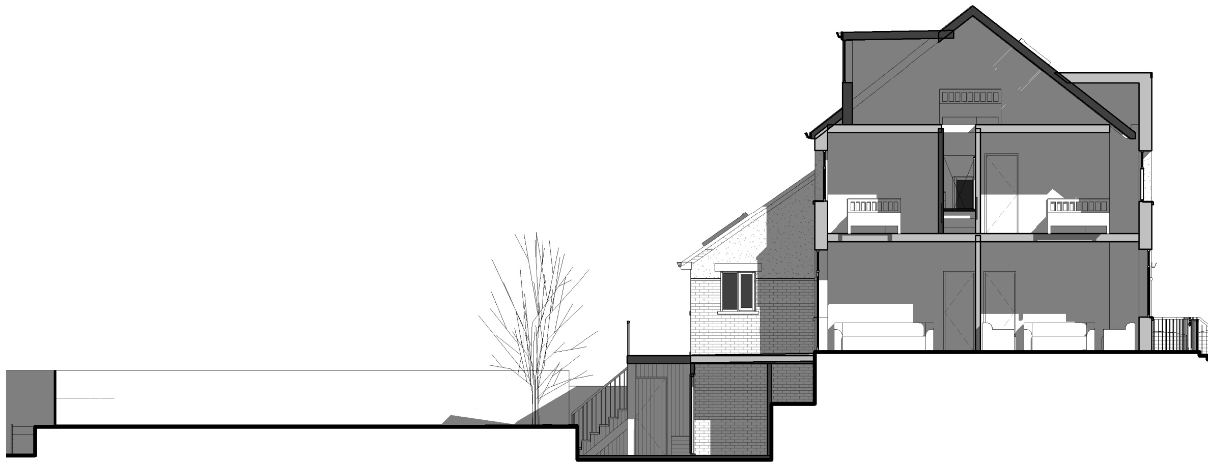
Elevation 03 - Proposed South Elevation 1 : 100
