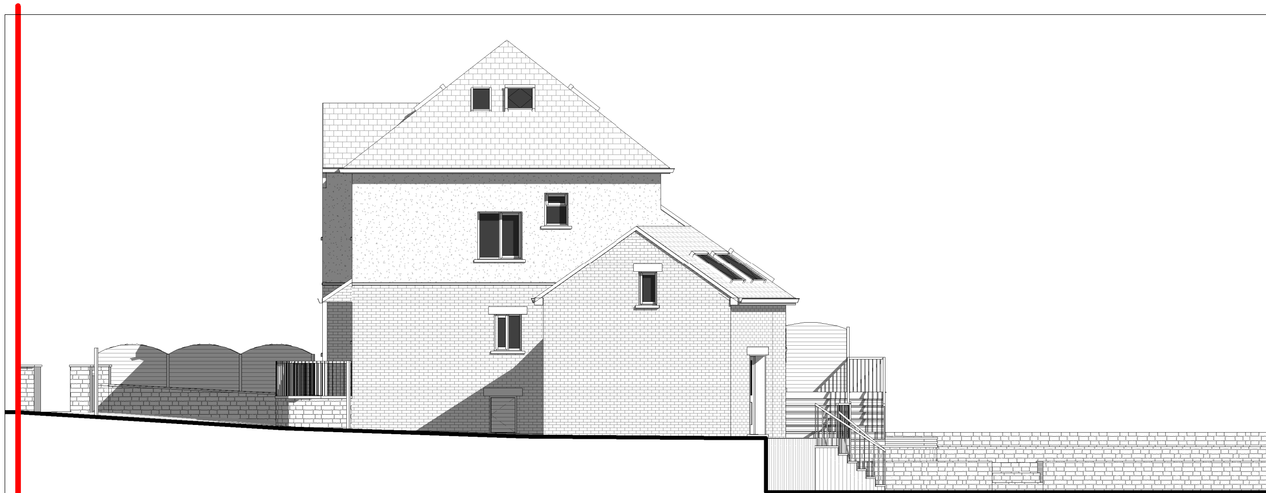
Elevation 01 - Existing North Elevation
