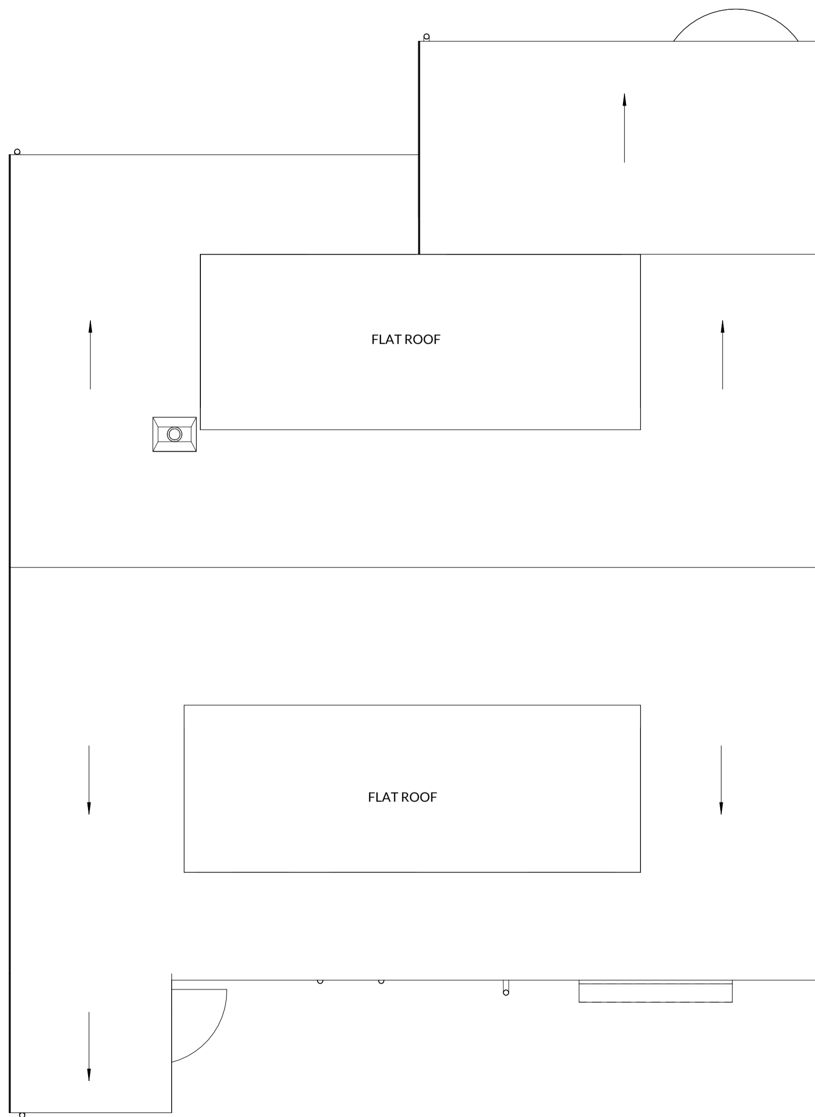
1 ROOF PLAN - AS EXISTING 1:50
