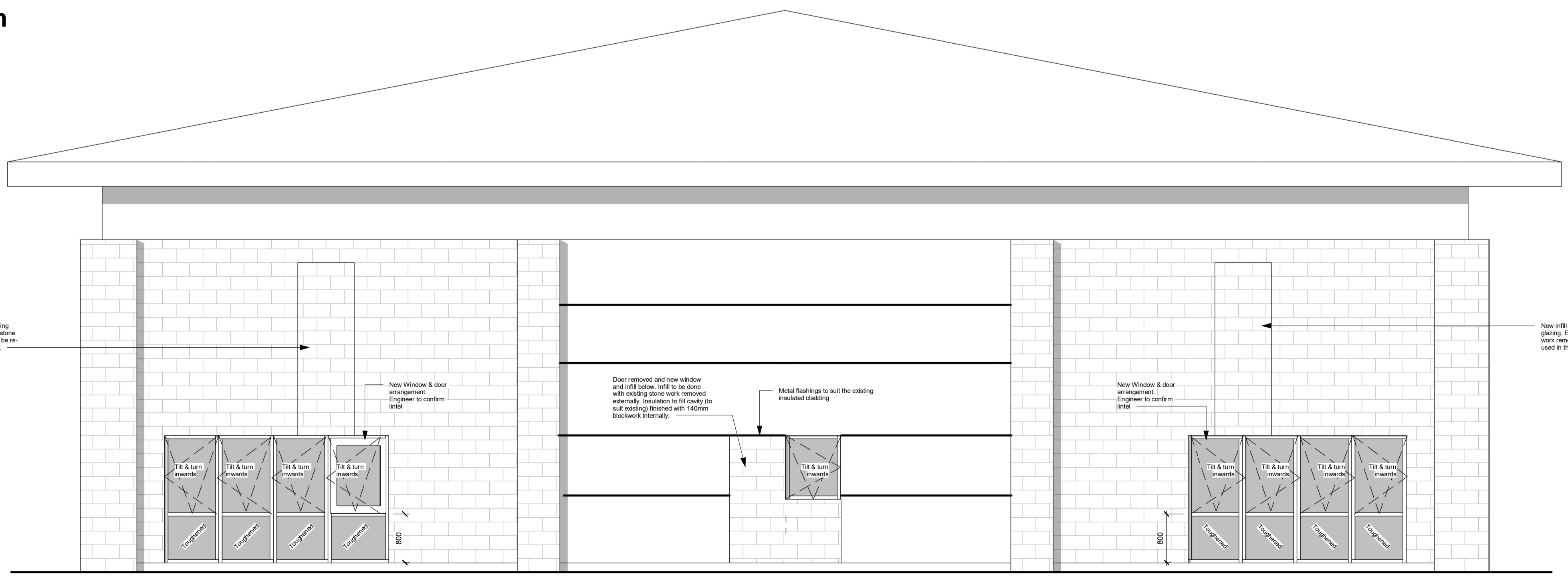
(working) East 1 : 50
