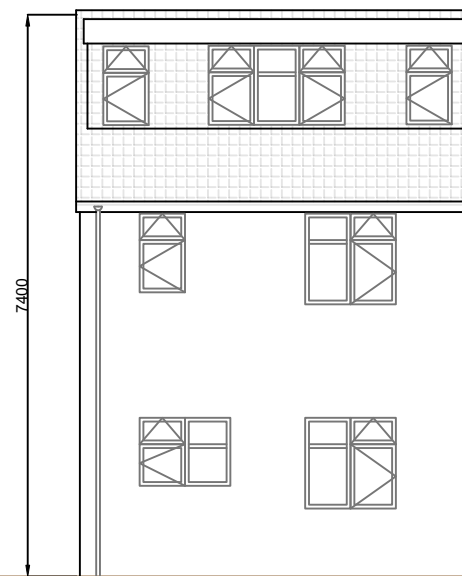
South Elevation
