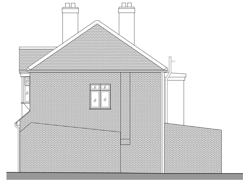
Side Elevation - View from "The Lord Nelson"
