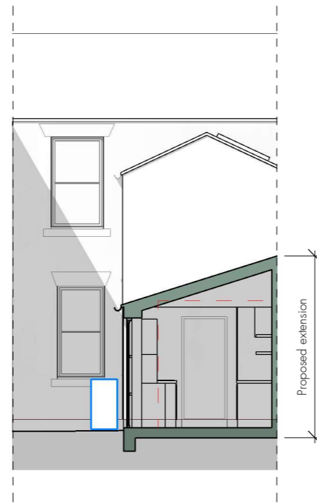
North Elevation as Proposed
