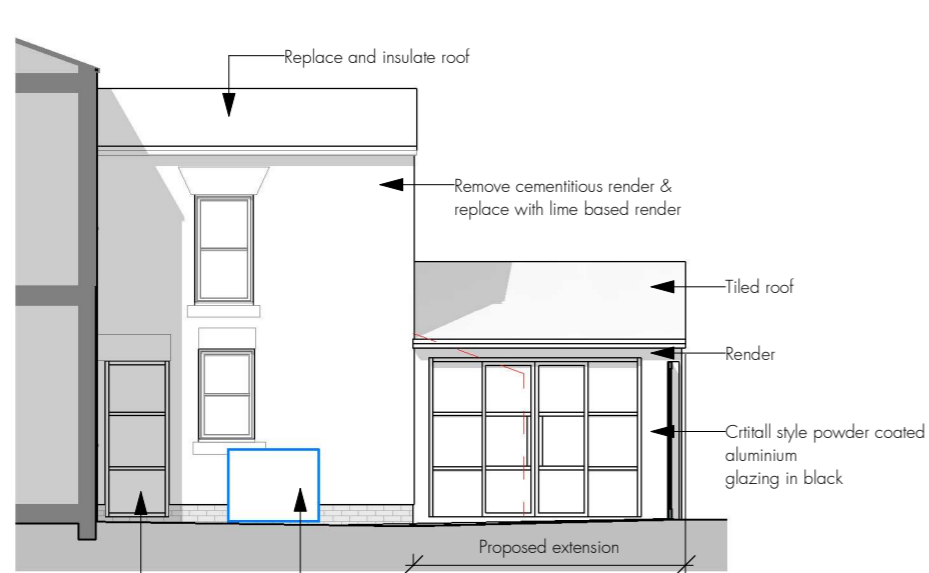
East Elevation as Proposed
