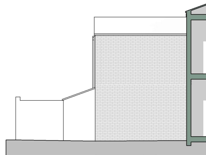
West Elevation as Existing
