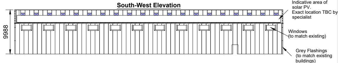
South-West Elevation
