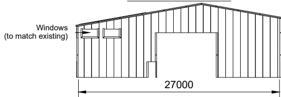
South-East Elevation
