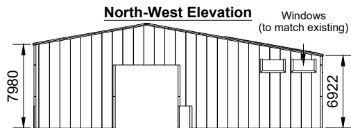
North-West Elevation
