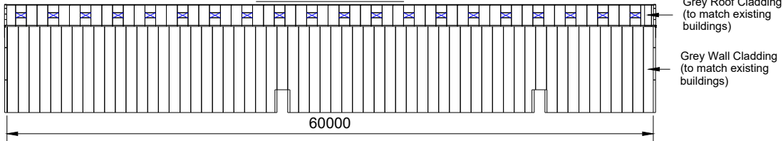
North-East Elevation
