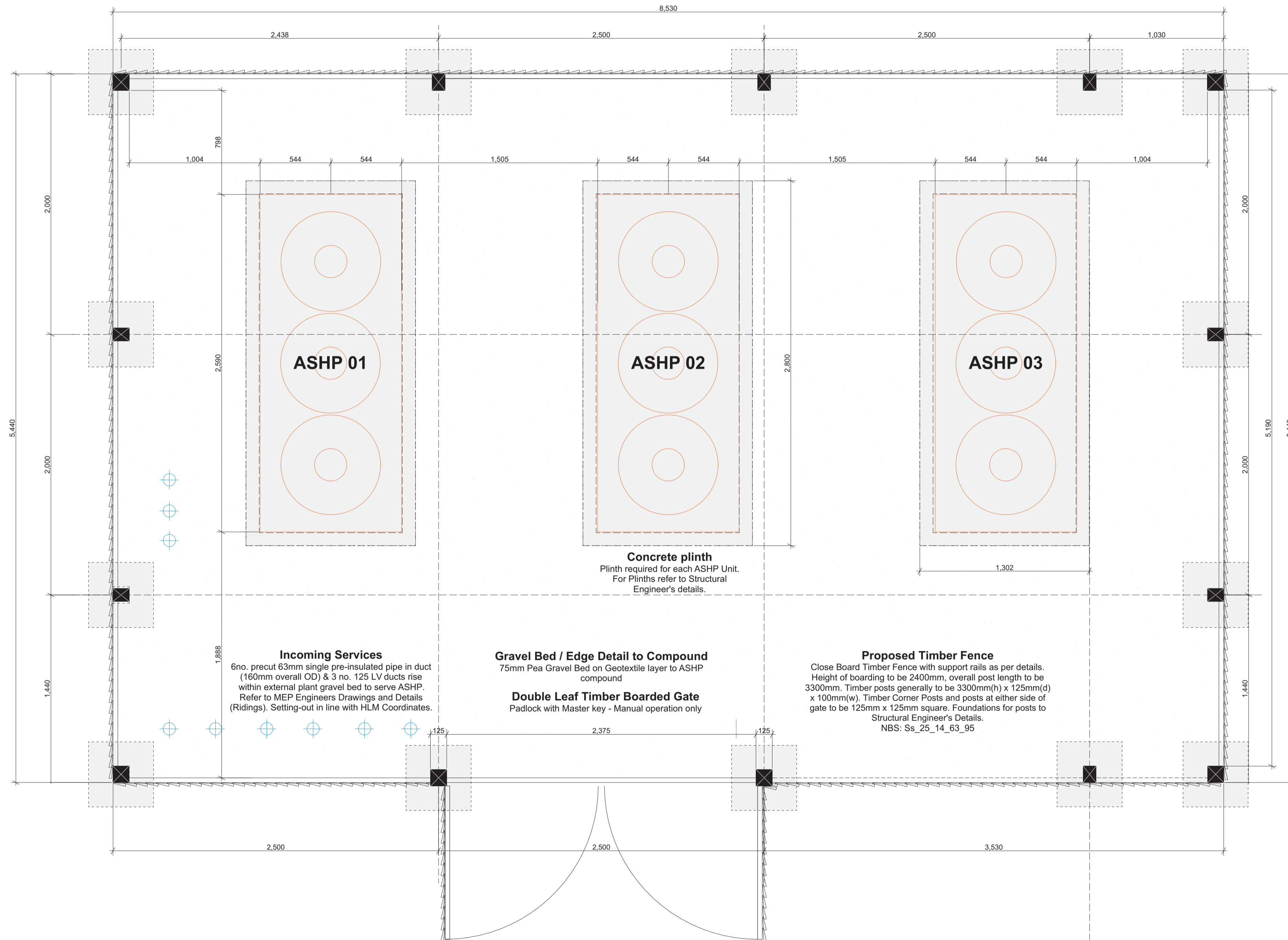
ASHP COMPOUND TIMBER FENCING DETAILS
