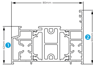
SP103 INTERMEDIATE FLUSH OUTER FRAME
