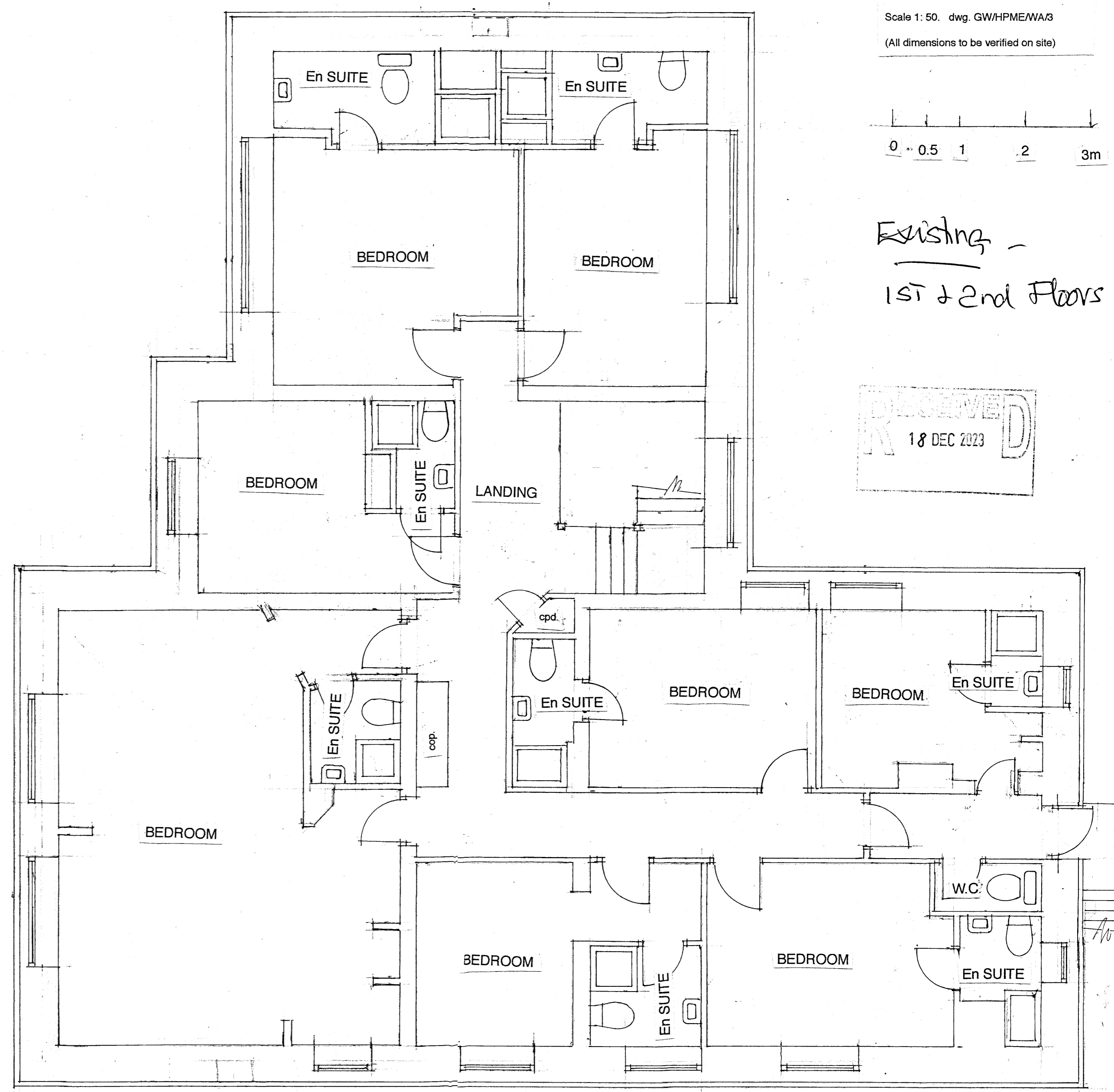
EXISTING SECOND FLOOR PLAN
