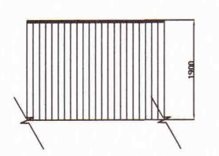
PART ELEVATION OF FENCE
